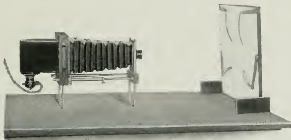
Fig. 82. Kodak Enlarging Outfit.
